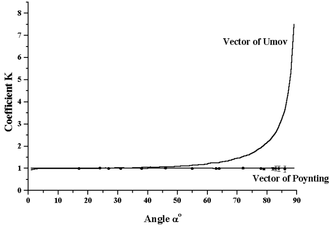
Fig. 6. The theoretical curves of the behavior of the coefficient \mathcal{K} versus angle according to the Poynting vector and according to the Umov vector and the experimental results for the case of the waves with parallel magnetic field vectors.
