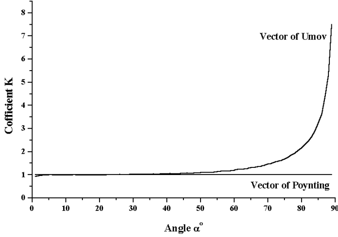
Fig. 2. Theoretical curves of the behavior of the coefficient K versus angle according to the Poynting and Umov vectors.
