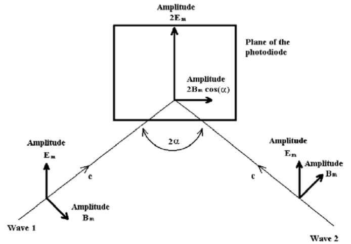
Fig. 4. Equivalent scheme of the experimental arrangement when the electric field vectors from the wave in the branch 1 are parallel to the electric field vectors from the wave in the branch 2, 2\alpha is the angle between straights connecting each of two sources with the centre of the sensor.
