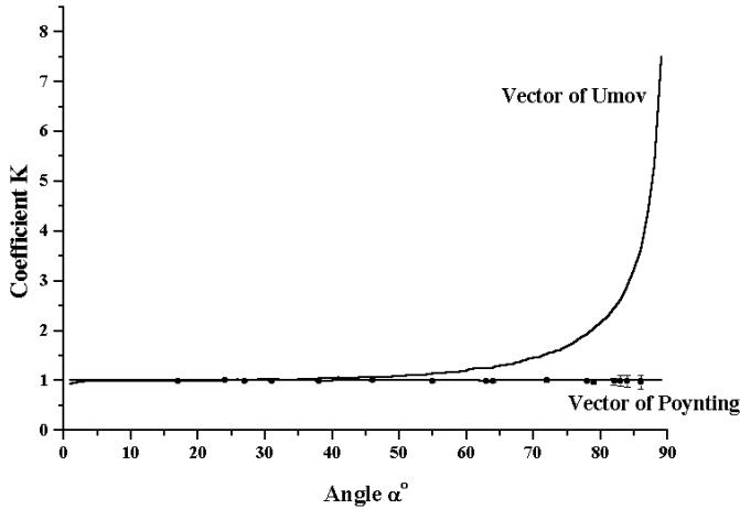
Fig. 7. The theoretical curves of the behavior of the coefficient \mathcal{K} versus angle according to the Poynting vector and according to the Umov vector and the experimental results for the case of the waves with parallel electric field vectors.
