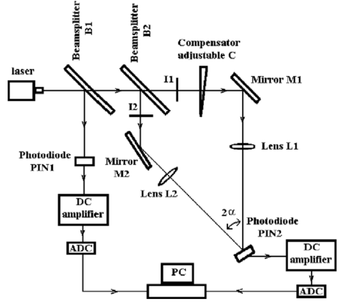
Fig. 3. The experimental arrangement diagram. I1 and I2 are optical obturators. ADC is the analog digital converter.
