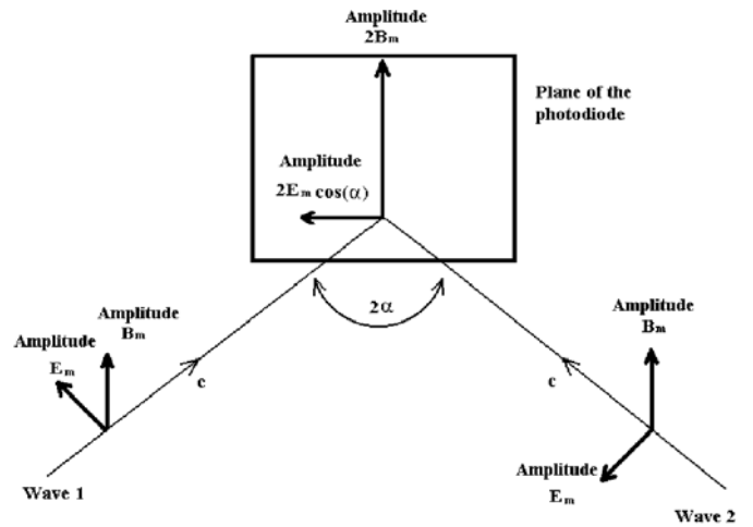
Fig. 5. Equivalent scheme of the experimental arrangement when the magnetic field vectors from the wave in the branch 1 are parallel to the magnetic field vectors from the wave in the branch 2.
